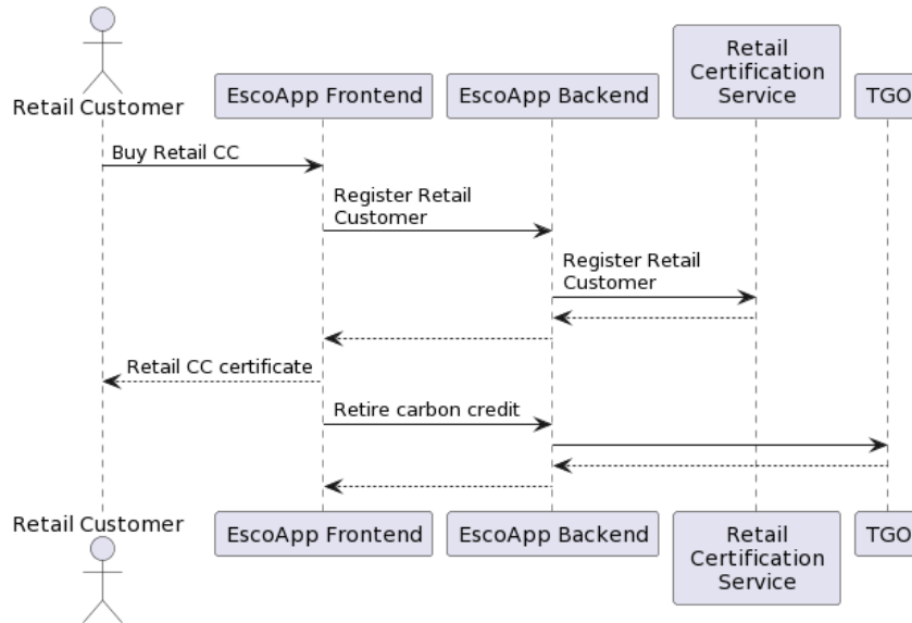
Fig 1 Sequence Diagram
